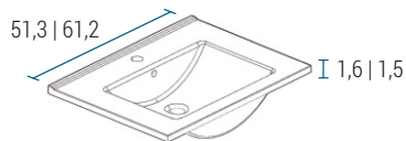
ML50SA | ML60SA
